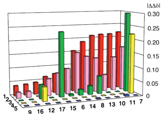
Figure 1. Comparison of the chiral discrimination abilities of 1–5. The absolute values of the chemical shift nonequivalences ( \Delta\Delta\delta ) observed for 6–17 are indicated by the height of the vertical bars. The conditions for the measurements are shown in the footnote of Table 1. The signals used for comparison were selected arbitrarily.
