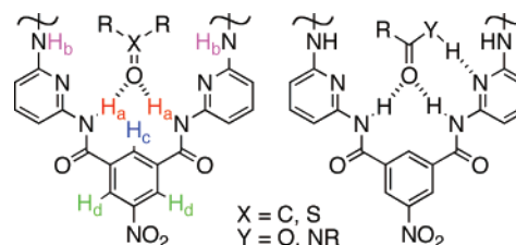
Figure 5. Double and triple hydrogen bonds between 1 and a guest molecule.
