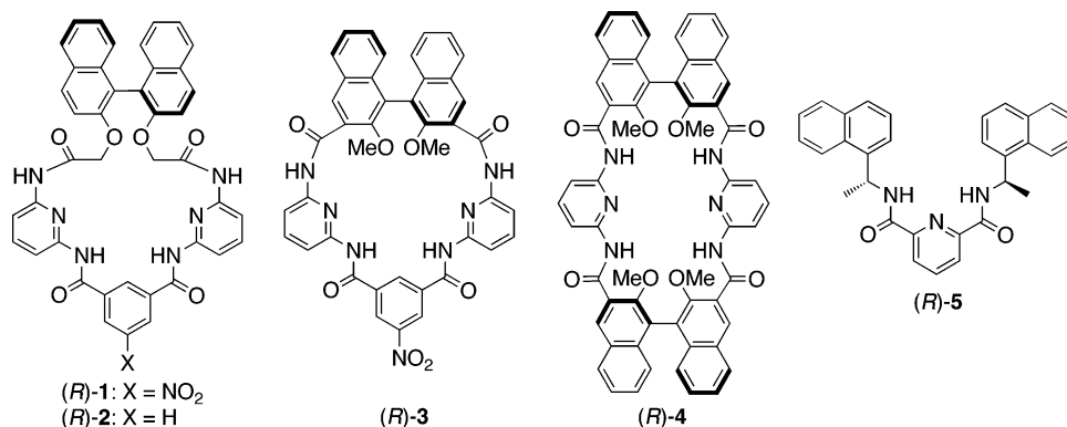
Chart 1. Chemical Structures of Reagents 1–5
