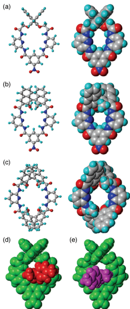
Figure 6. Optimized structures for (a) ( R )- 1 , (b) ( R )- 3 , (c) ( R )- 4 , (d) ( R )- 1 –( S )- 13 complex, and (e) ( R )- 1 –( R )- 13 complex. In (d) and (e), ( R )- 1 is shown in green, and ( S )- 13 and ( R )- 13 are shown in red and magenta, respectively. The geometries were optimized at the HF/6-31G* level using Gaussian 98W (Gaussian Inc.) and were drawn with Sybyl 6.4 (Tripos Inc.).
