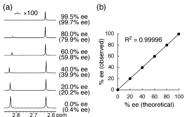
Figure 2. (a) A selected region of 600 MHz 1 H NMR of ( S )- 13 (1.4 mg, 15 mM) with various enantiomeric purities in the presence of ( R )- 1 (6.7 mg, 15 mM) in CDCl 3 (0.6 mL) at 22 °C. Observed % ee values calculated from the integrals are indicated in the parentheses. (b) Correlation between the theoretical and observed % ee values.
