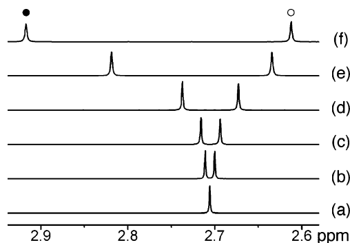
Figure 3. 600 MHz 1 H NMR of rac - 13 (277 μg, 3 mM) in the presence of ( R )- 1 (0–15 mM) in CDCl 3 (0.6 mL) at 22 °C. ( R )- 1 : (a) no addition; (b) 5 mol % (69 μg); (c) 10 mol %; (d) 30 mol %; (e) 100 mol %; (f) 500 mol %. Filled and open circles represent ( R )- and ( S )-enantiomers, respectively.
