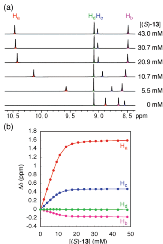
Figure 4. (a) Complexation-induced shifts (Δδ) for the H a –H d protons of ( R )- 1 (12 mM) as a function of [( S )- 13 ] in CDCl 3 at 22 °C. (b) Plots of the complexation-induced shifts (Δδ) for the H a –H d protons of ( R )- 1 as a function of [( S )- 13 ].
